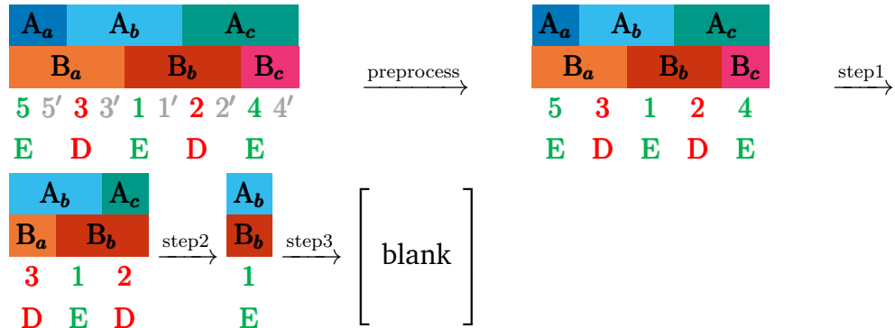
Figure 6.7: Complete trace of the algorithm running on the example.
